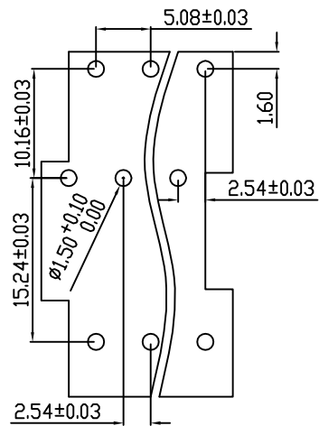
PCB Layout
