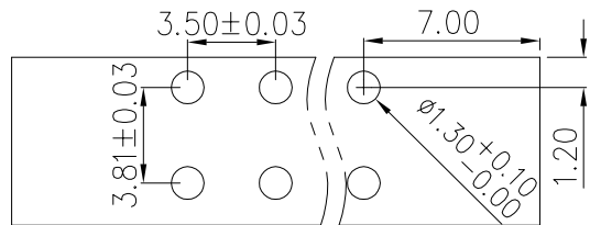
PCB LAYOUT
